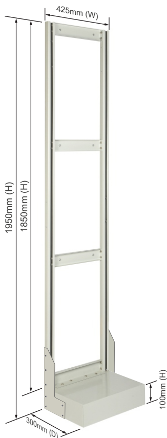
Single Sided Stand for Roo Tilt Bins Size : 425mm(W) x 1950mm(H) x 300mm(D) Consists of :
