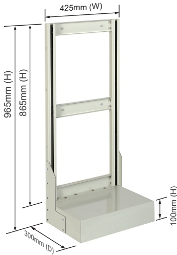
Single Sided Stand for Roo Tilt Bins Size : 425mm(W) x 965mm(H) x 300mm(D) Consists of :
