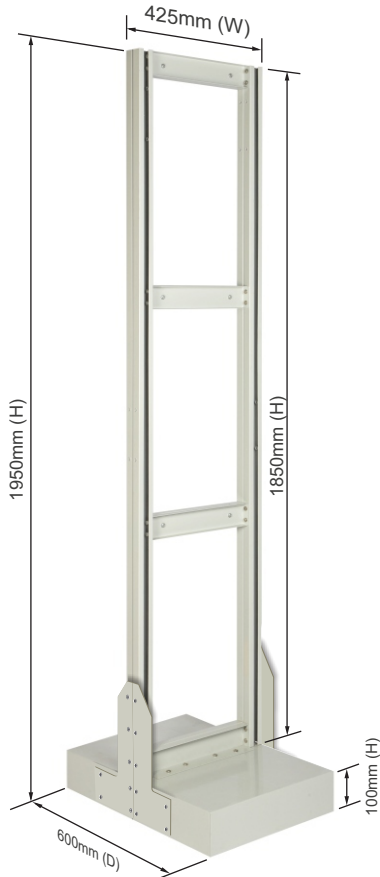
Double Sided Stand for Roo Tilt Bins Size : 425mm(W) x 1950mm(H) x 600mm(D) Consists of :
