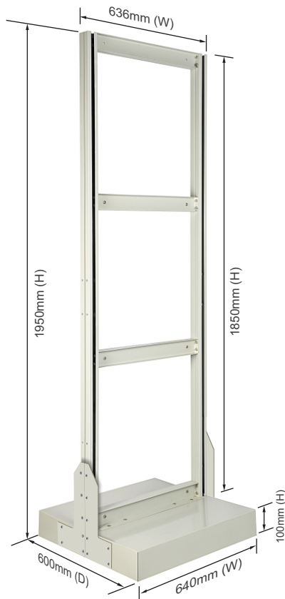
Double Sided Stand for Roo Tilt Bins Size : 640mm(W) x 1950mm(H) x 600mm(D) Consists of :
