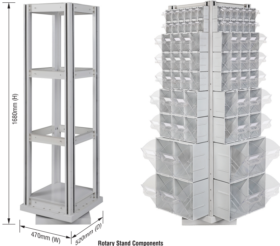
Rotary Stand Components
