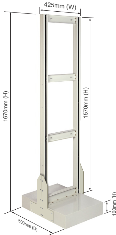
Double Sided Stand for Roo Tilt Bins Size : 425mm(W) x 1670mm(H) x 600mm(D) Consists of :
