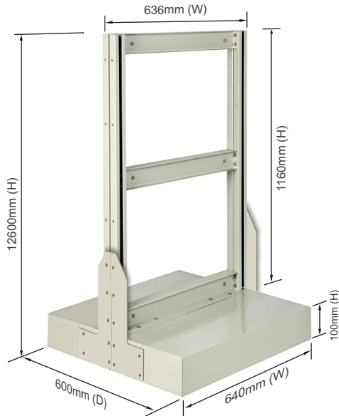
Double Sided Stand for Roo Tilt Bins Size : 640mm(W) x 1260mm(H) x 600mm(D) Consists of :
